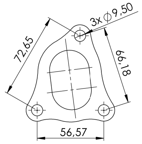
Flange "160A" Sp.8 mm
